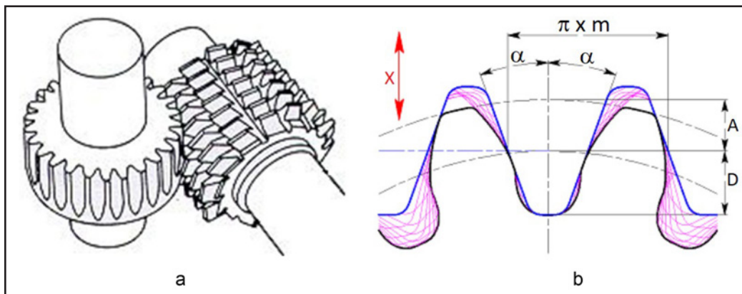
Figure 1 a – metal gear hobbing; b – definition of the gear profile by rack generation; m – module; \alpha – rack profile (pressure) angle; A – gear tooth addendum; D – gear tooth dedendum; X – addendum modification or X-shift.
